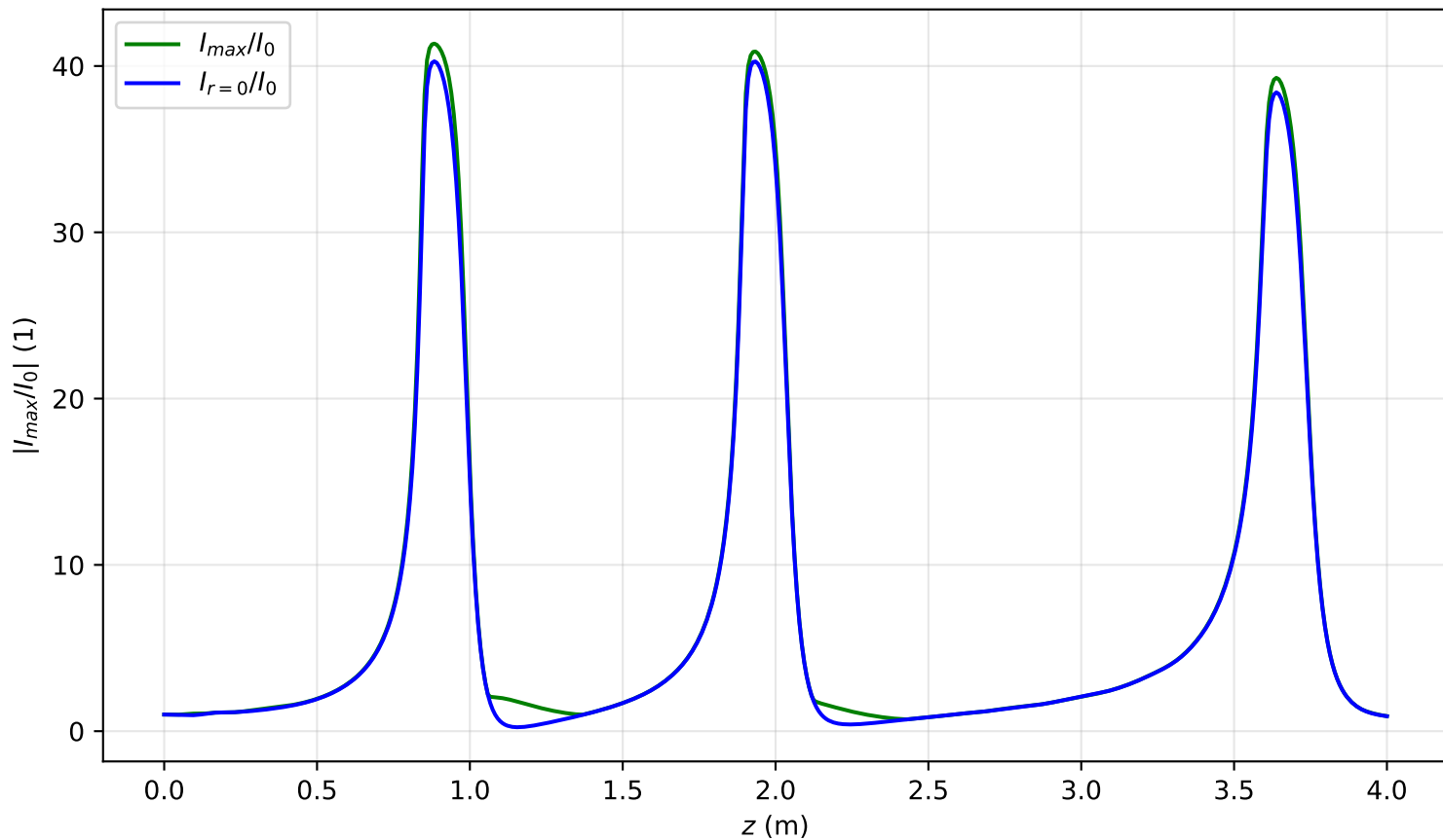
I_{max}(x=0, y=0, z)/I_0 , P_{in}=2.6P_{cr} , noisy input, artificial time
